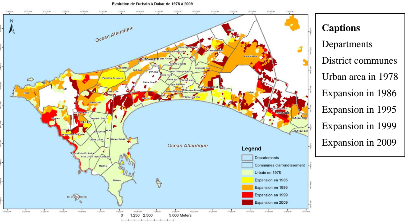
Figure 2: extension of the built-up area of the city of Dakar between 1978 and 2009 (Source: Instituto Agronomico per l'Oltremare and EC-JRS)
