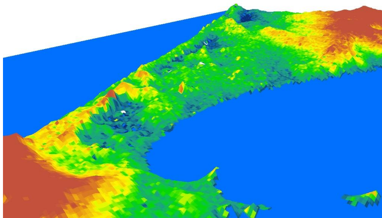
Figure 3: 3D figure of the topographic profile of the various drainage basins in the departments of Pikine and Guédiawaye (Digital Terrain Model, Extract from a presentation on the "Contribution to the identification of flood causes and solutions", Directorate of Water Resources Management and Planning, 2009)
