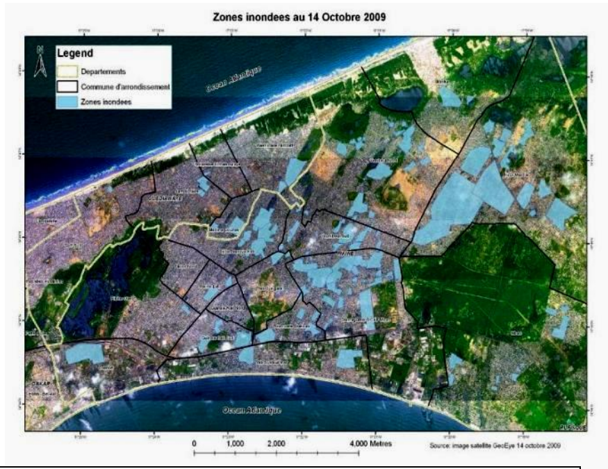
Figure 1: distribution of flood zones in the area studied (Source: GeoEye image of October 14, 2009)
